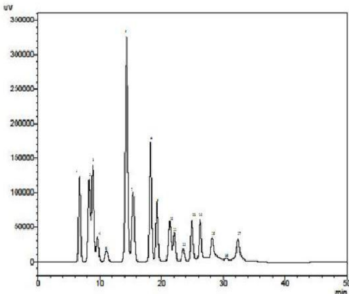
Spectra.1: Standard amino acid spectra of aspartic acid, threonine, serine, glutamic acid, proline, glycine, alanine, cysteine, valine, methionine, isoleucine, leucine, tyrosine, phenyl alanine, histidine, lysine, arginine and glutamic acid.
