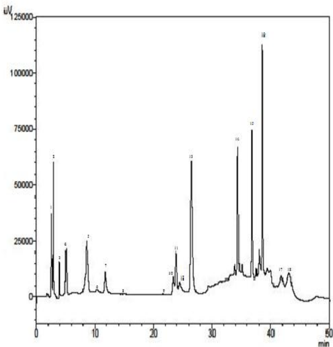
Spectra. 2: Chlorogenic acid, imidazol, gallic acid, quinine, hydraquinone, catachin hydrate, vanillin, epigallactocatechin, rutin, naringenin, quercetin, naringin, couymarin, indole, 2-methyl naphthaquinone, hydorxy diphenyl phenol, cucumin, quinine, quinoline, tannic acid standard HPLC spectra
